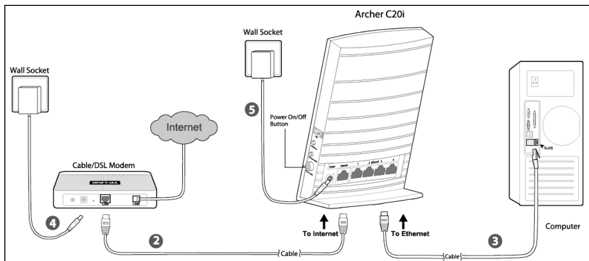
Figure 2-1 Hardware Installation
