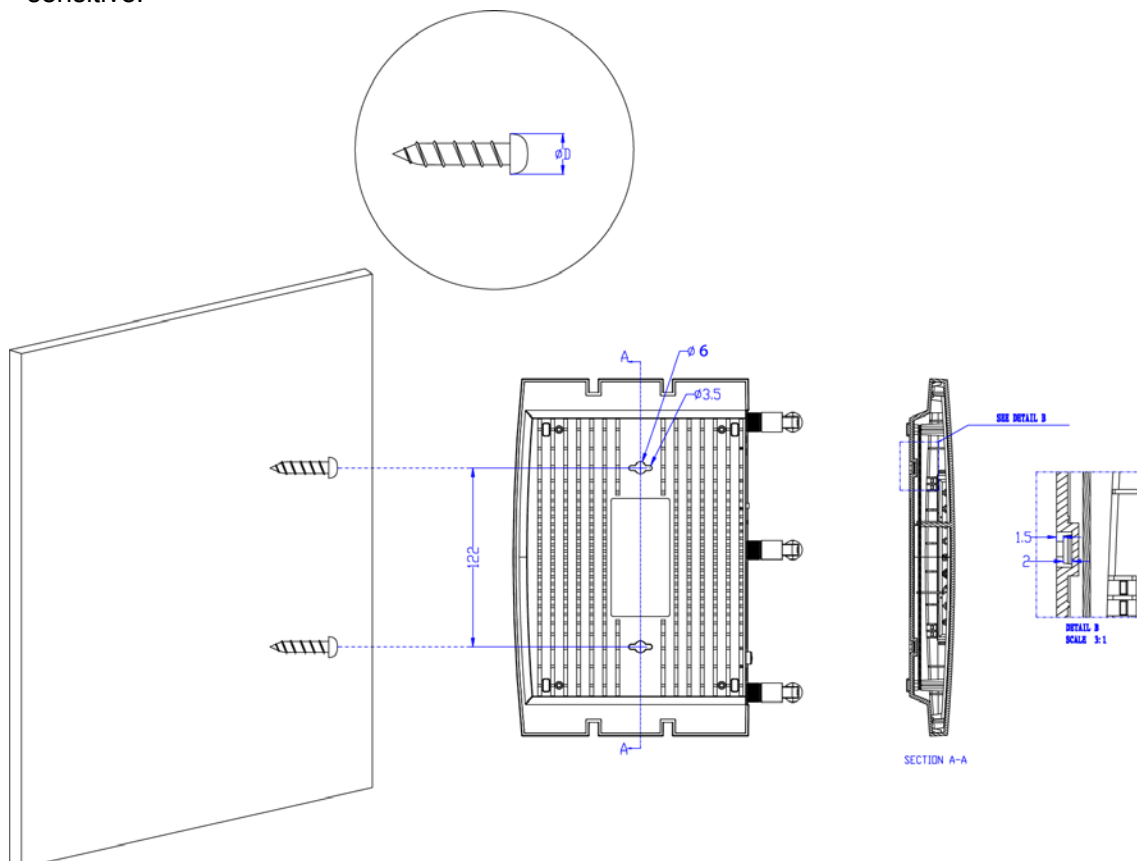
Figure 2-1 Wall-mount install
